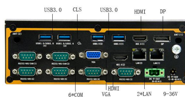
Rear IO View
