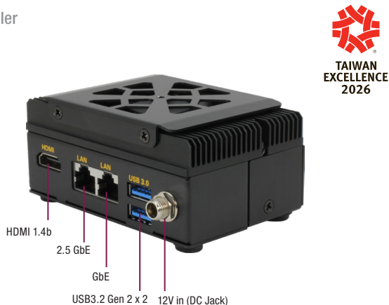
With Heatsink
