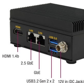
With Heatsink
