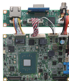
▲ Assembly view
